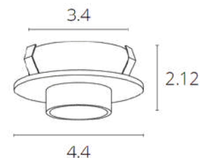
A6182PL-1BK – 4000K A6382PL-1BK – 3000K LED | 2W | 150Lm
