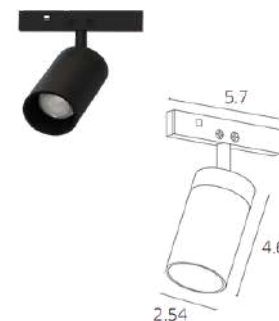
A6227PL-1BK – 4000K A6327PL-1BK – 3000K LED | 2W | 150Lm
