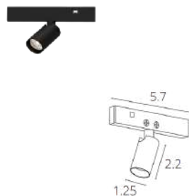
A6226PL-1BK – 4000K A6326PL-1BK – 3000K LED | 1W | 65Lm
