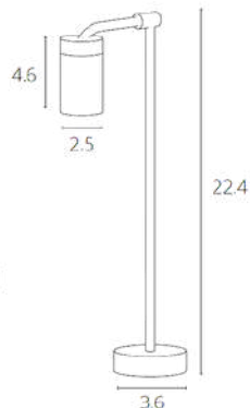
A6196LT-1BK – 4000K A6396LT-1BK – 3000K LED | 2W | 135Lm
