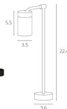
A6197LT-1BK – 4000K A6397LT-1BK – 3000K LED | 5W | 275Lm
