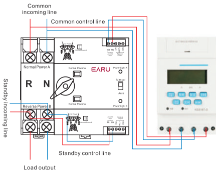
Timing switching connection mode
