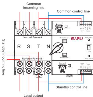
Timing switching connection mode
