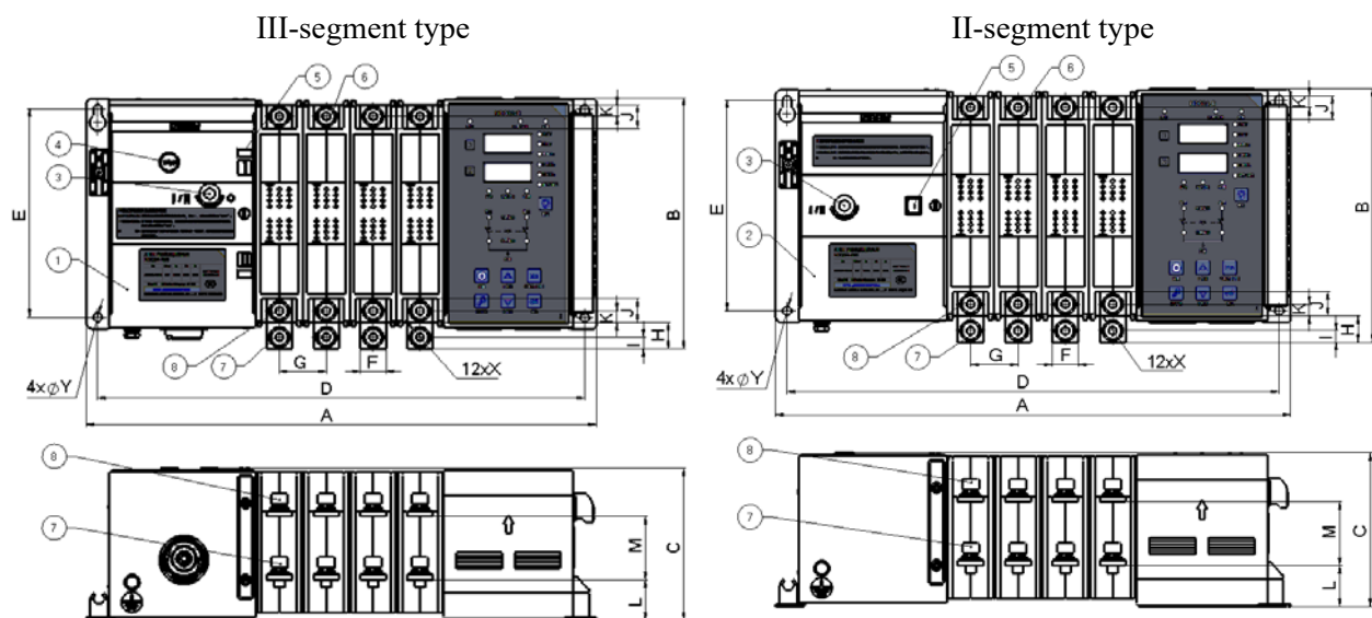
Fig. 1 External dimensions and installation dimensions of integral switch
