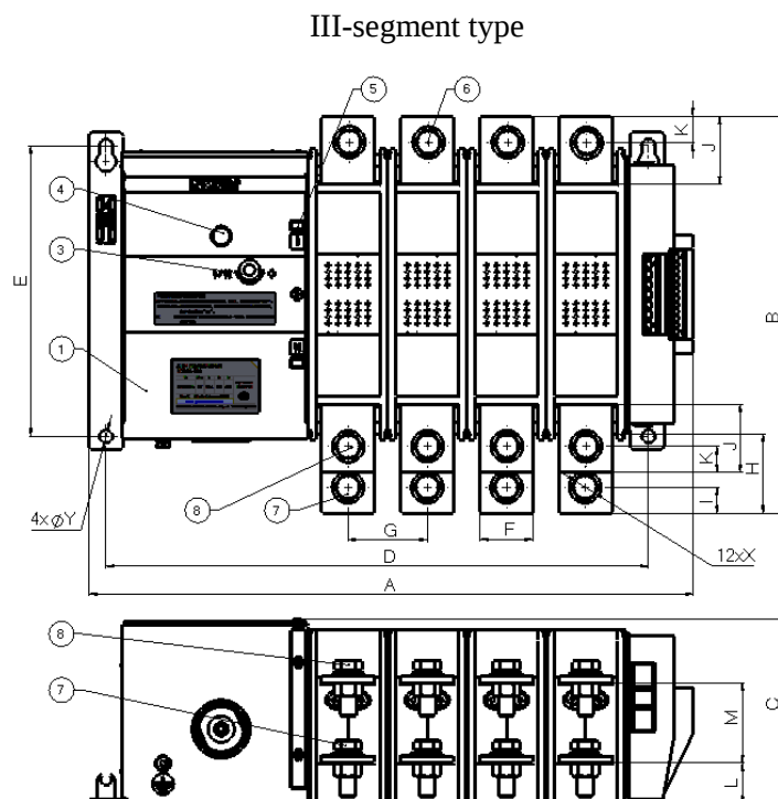
Fig. 2 External dimensions and installation dimensions of mechanism body of split switches
