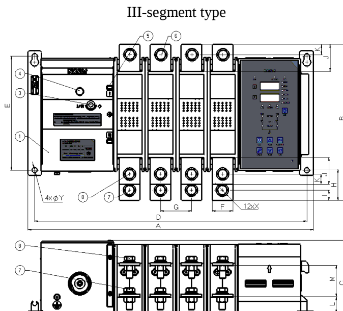
Fig. 1 External dimensions and installation dimensions of integral switch
