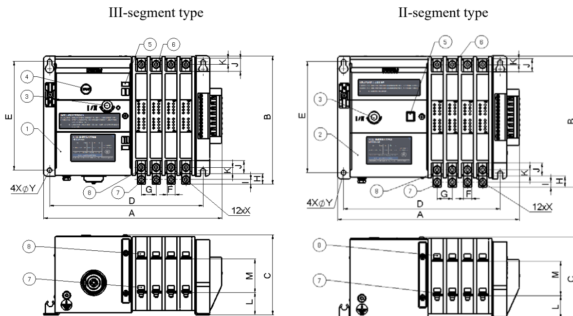
Fig. 2 External dimensions and installation dimensions of mechanism body of split switches
