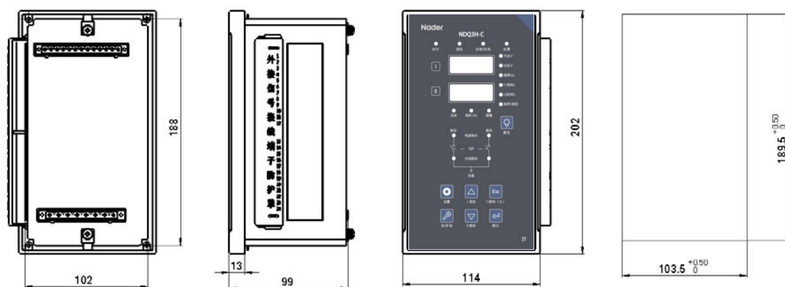
Note: The dimensions of Type A/B/C/D split controllers are all the same. Therefore, only one dimension chart is attached here. The limit deviation of the unspecified tolerance dimension shall comply with GB/T 1804-C.
