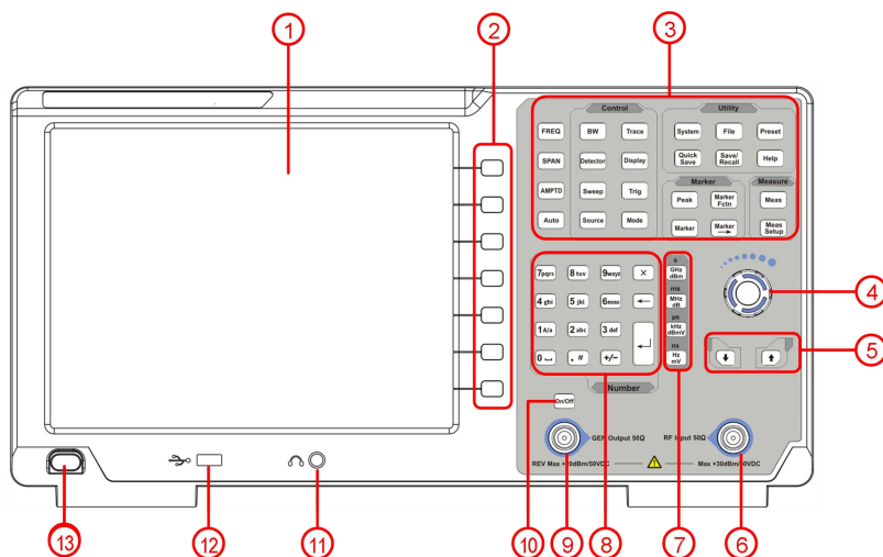
Figure 4- 1 Front panel
