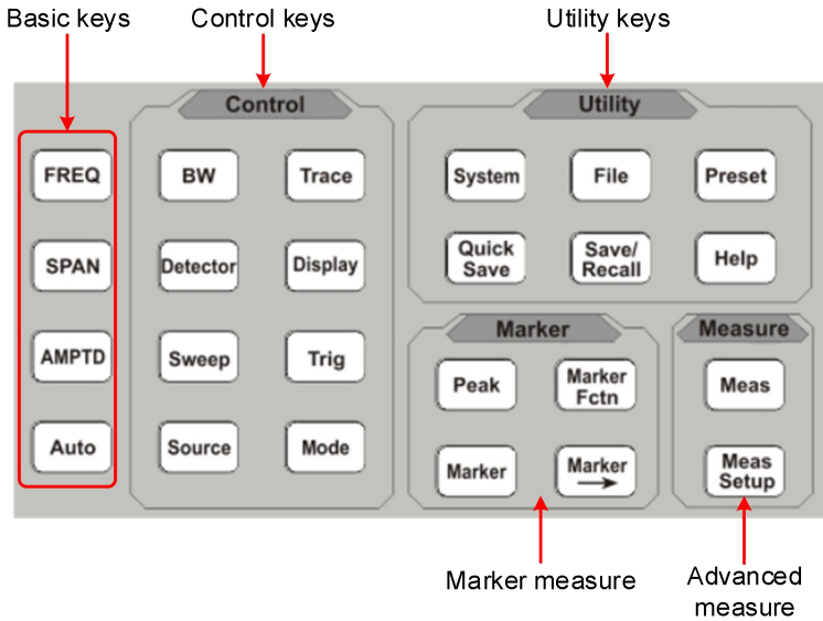
Figure 4- 2 Function Keys
