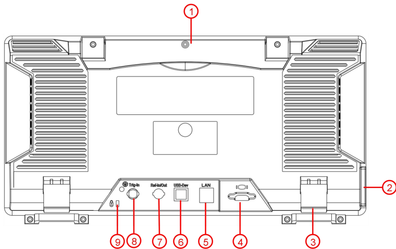
Figure 4- 6 Rear Panel
