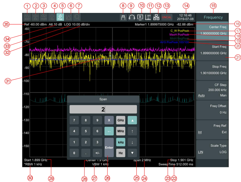
Figure 4- 7 User interface
