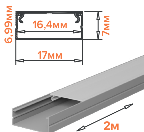
WAP-S-16/7/2000-A-LITE
