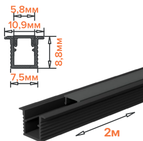
WAP-S-11/9/2000-B
