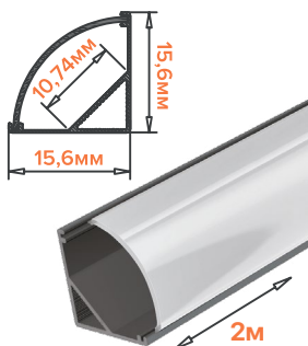
WAP-S-16/16/-A-LITE
