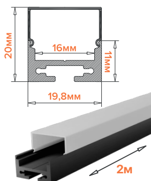
WAP-S/H-20/20/2000-BW
