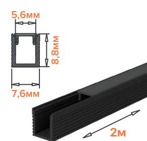
WAP-S-8/9/2000-B
