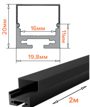
WAP-S/H-20/20/2000-B
