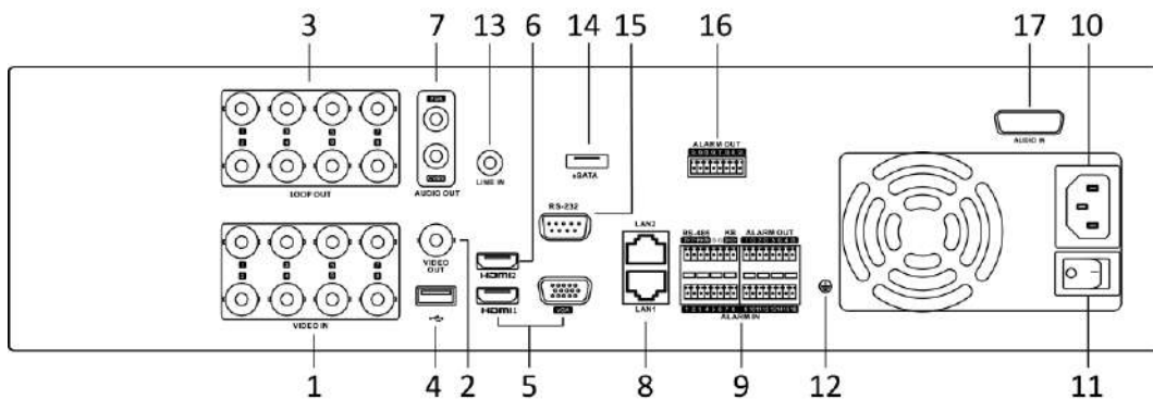
Figure 1-17 Rear Panel of DS-9000HUHI-K8 (with 8 Video Inputs)
