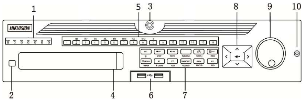
Figure 1-4 Front Panel of DS-9000HUHI/HTHI-K8 and iDS-9016HUHI-K8/16S
