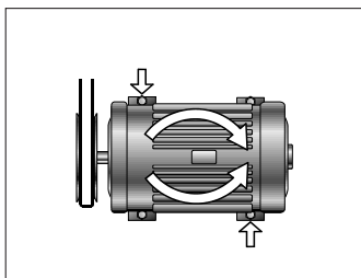
Fig 12 Horizontal angle alignment
