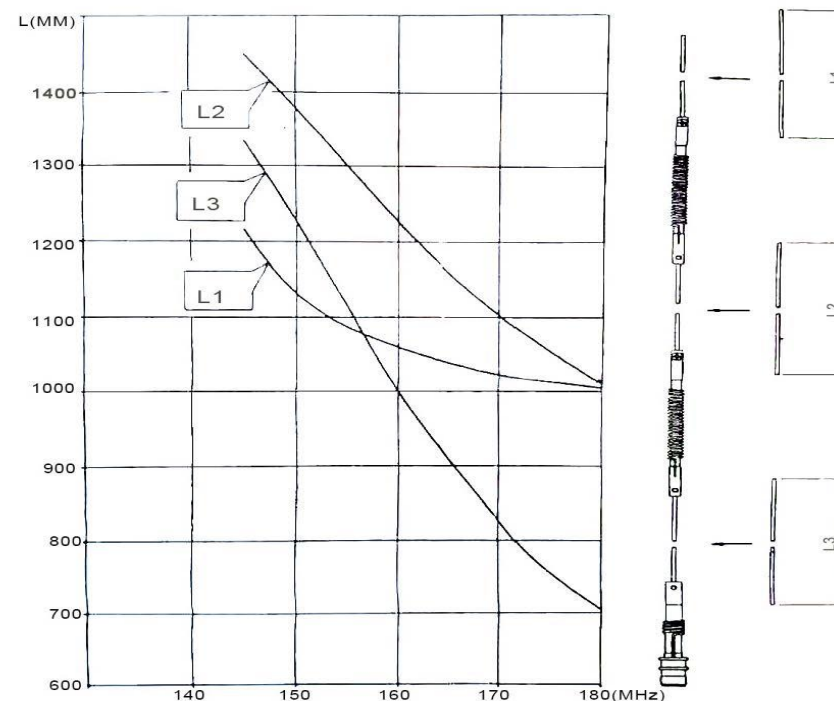
SIRUS F23 CUTTING CHART
