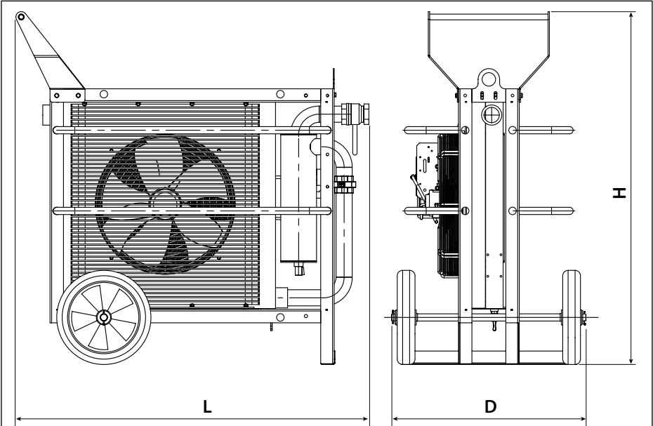
Fig. 2.3 Dimensions, mass of aftercooler
