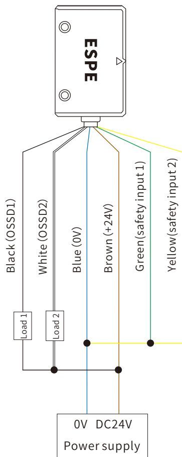
SSR2101 Standard mode(NPN)
