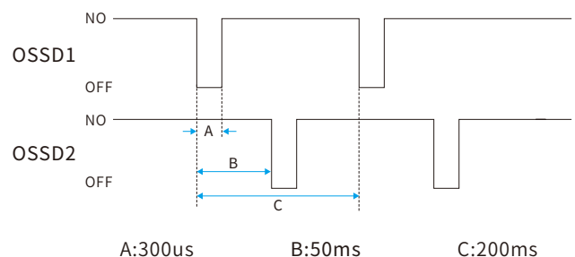
PNP output timing diagram
