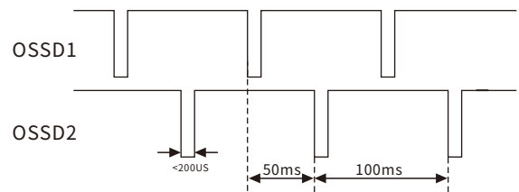
PNP timing chart
