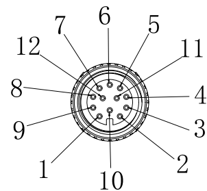
M12 waterproof aerial female connector Advanced series
