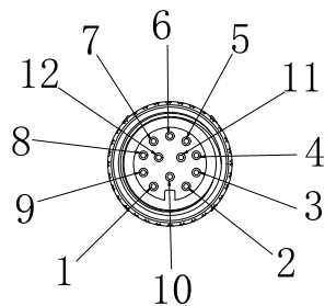
M12 waterproof aviation female connector
