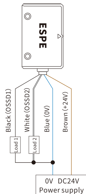
SSR2100 Basic mode (PNP)
