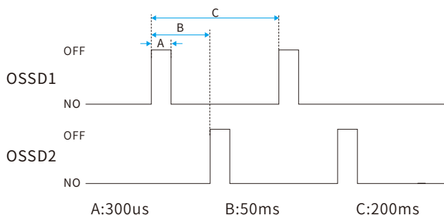
NPN output timing diagram
