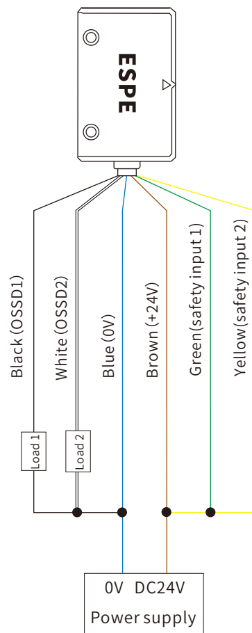
SSR2101 Standard mode(PNP)
