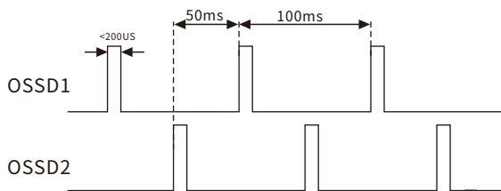
NPN timing chart
