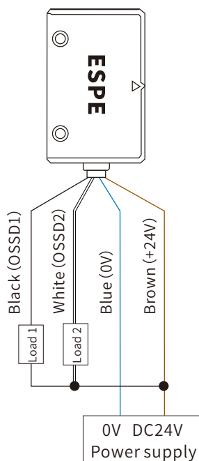
SSR2100 Basic mode (NPN)
