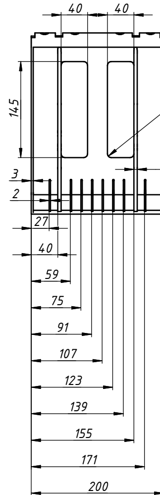
A (1:4)
