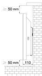
Figure 11. Dimensions of the convecter after assembly
