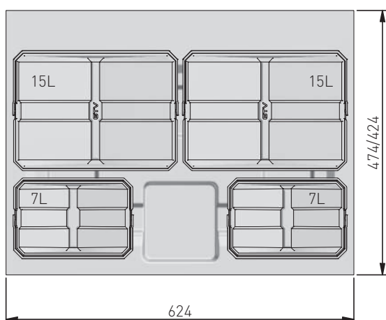
PB-AS-800-2X15L-2X7L-45
