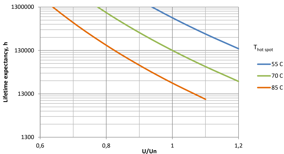
LIFETIME EXPECTANCY VS HOT SPOT TEMPERATURE AND VOLTAGE
