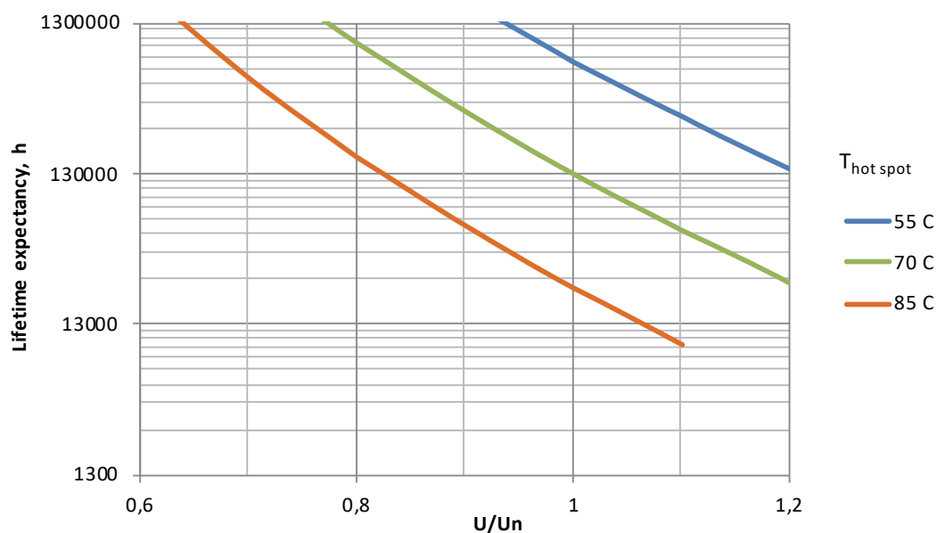
LIFETIME EXPECTANCY VS HOT SPOT TEMPERATURE AND VOLTAGE
