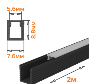
WAP-S-8/9/2000-B
