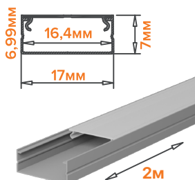
WAP-S-16/7/2000-A-LITE
