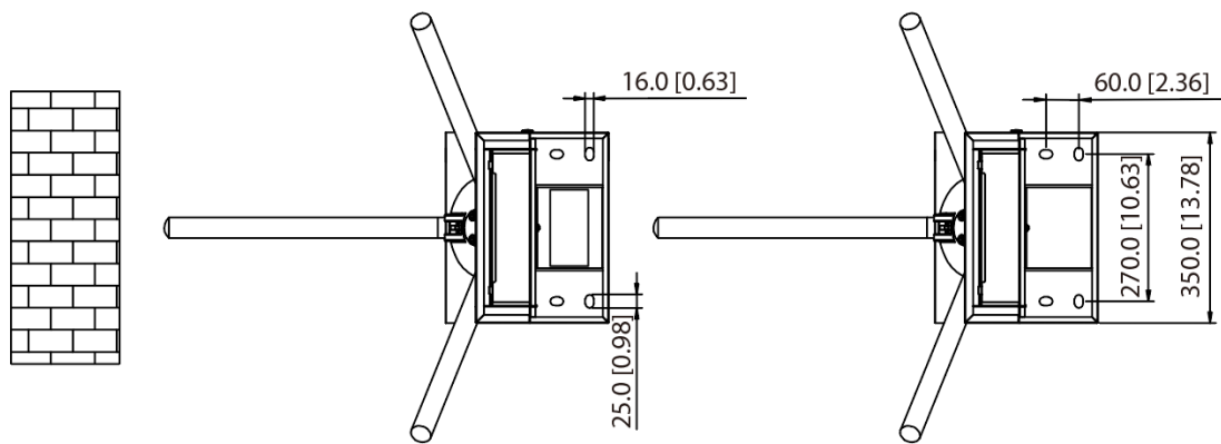
Figure 2-2 Hole drilling diagram (mm [inch])
