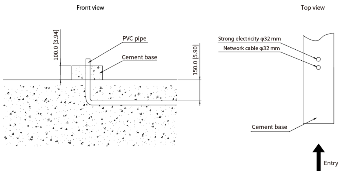
Figure 2-6 Wiring diagram
