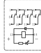
4 Form C (With LED and Diode D2) 四组转换(带LED与续流二极管 D2)
