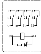
4 Form C (With LED) 四组转换(带LED)
