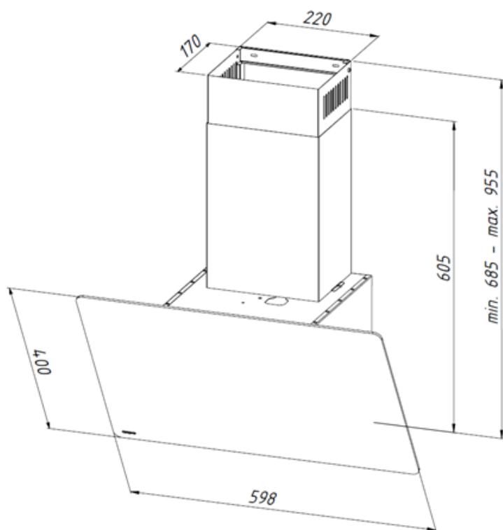
WK-4 Smart eco 60 cm
