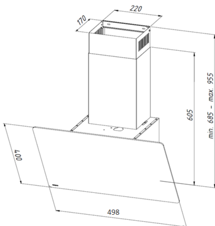
WK-4 Smart eco 50 cm
