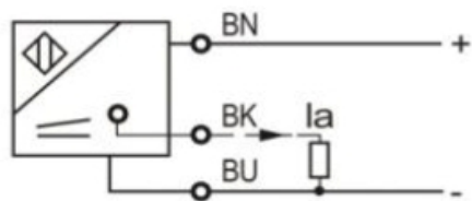
Current output
