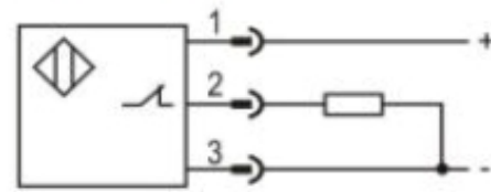
PNP NC
