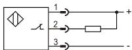
NPN NC
