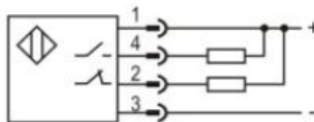
NPN NO+NC
