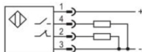
PNP NO+NC
