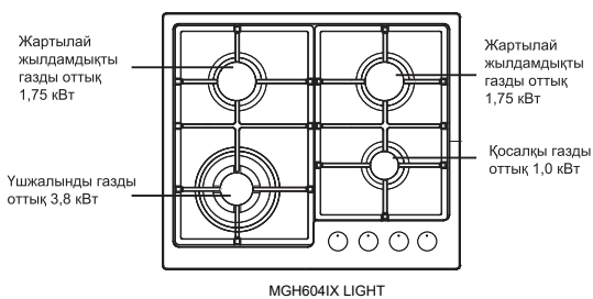
MGH604IX LIGHT
