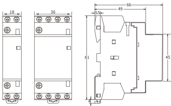
MCON21B 16/20/25A
