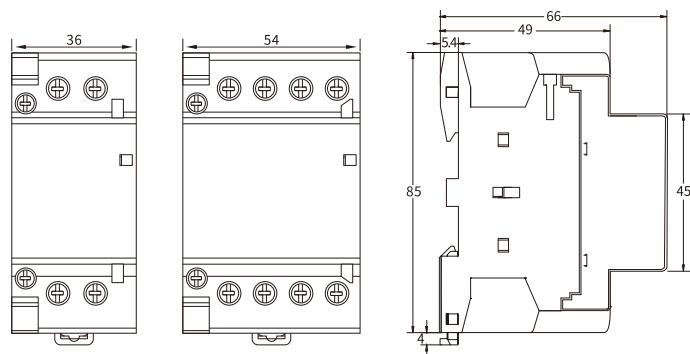
MCON21B 32/40/63A
