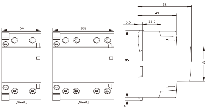
MCON21B 80/100/125A
