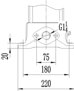
OVAL FLANGE
