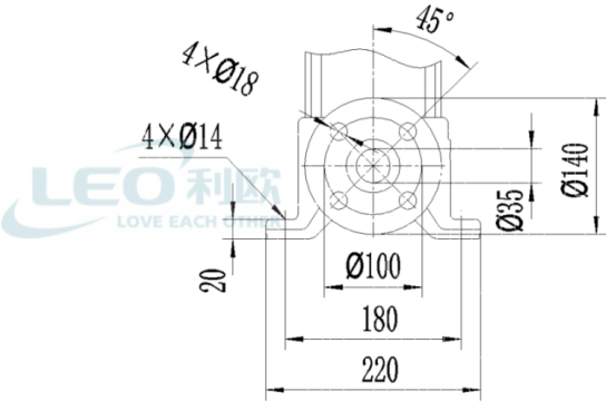
OVAL FLANGE
