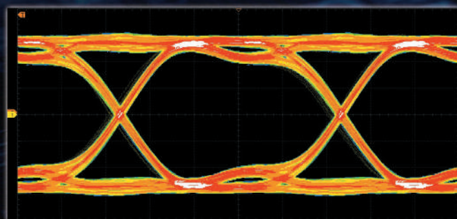
Use the 600 MHz bandwidth and 2 GHz bandwidth model respectively to perform eye measurement on the 1 Gb/s signal.
