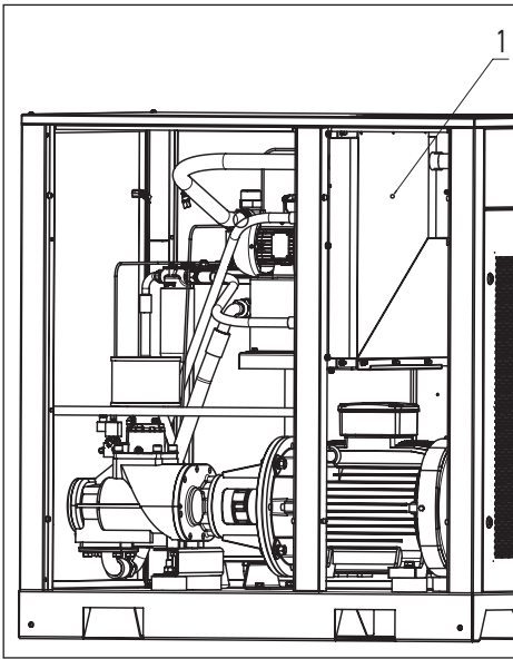
Fig. 5.6 Cleaning radiator
