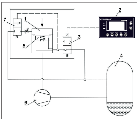
Fig. 2.5 Regulating system
