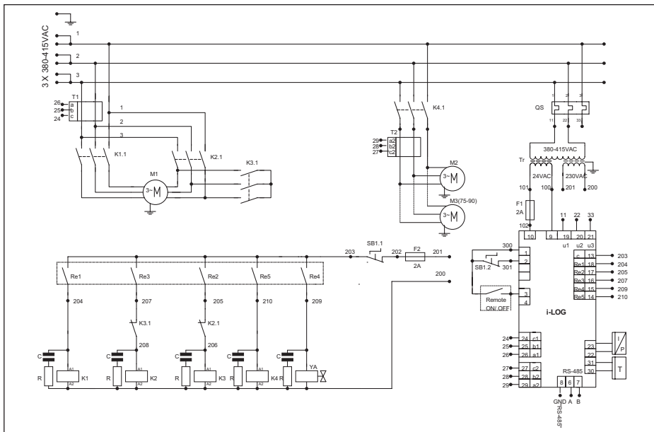
Fig. 2.6 Electrical diagram D30-D55
