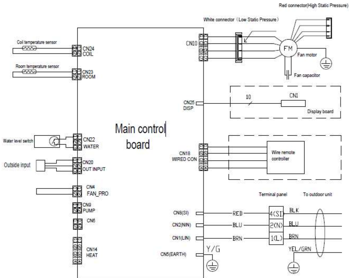
Electric wiring diagram 1820993.D
