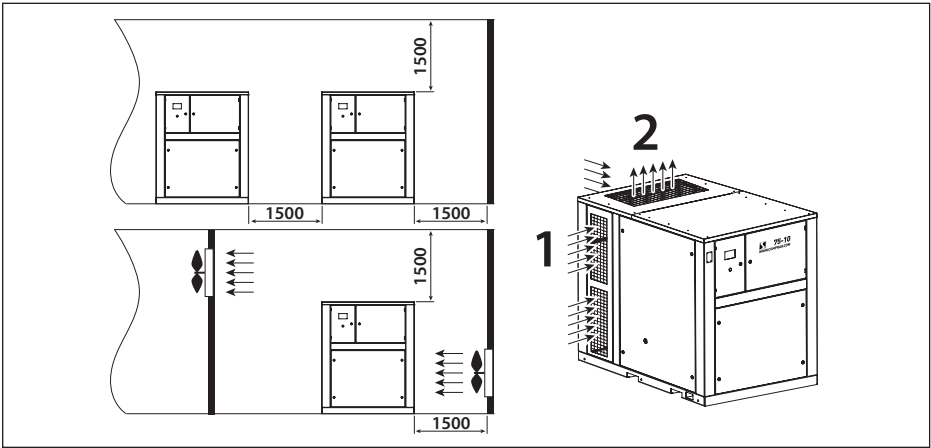
Fig. 3.3 Installation facility proposal A75 – 90.
