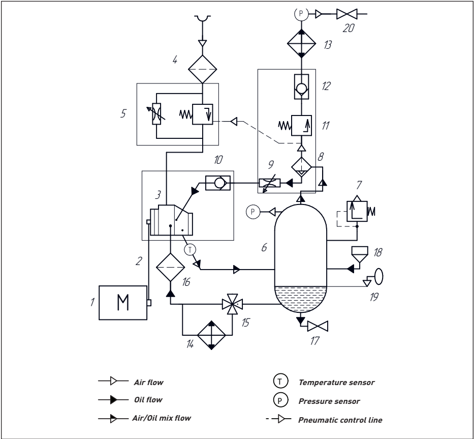
Fig. 2.3 Function diagram A75-90
