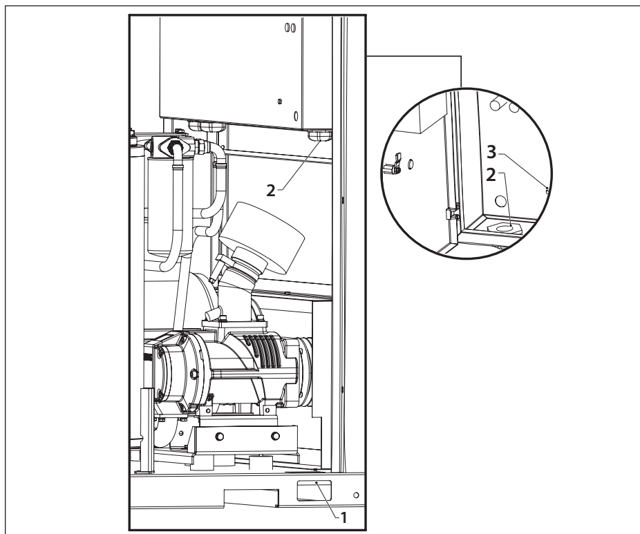
Fig. 3.5 Power cable connection
