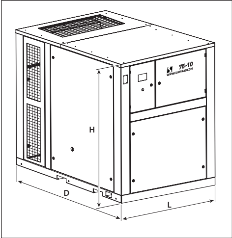
Fig. 3.2 Dimension drawing A75 – 90.
