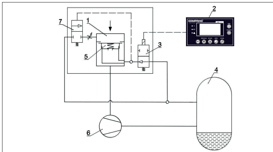
Fig. 2.5 Regulating system
