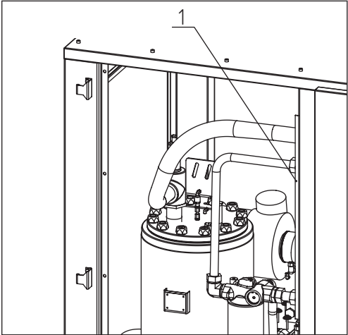
Fig 5.6. Cleaning radiator
