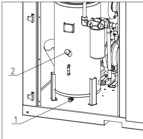
Fig. 5.3.1 Oil replacing
