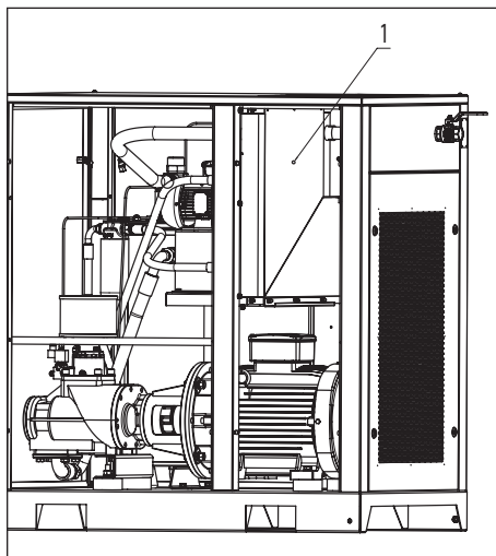
Fig. 5.6 Cleaning radiator
