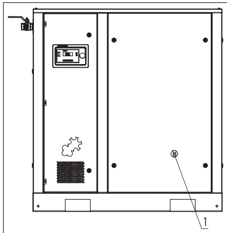
Fig. 5.2 Checking oil level
