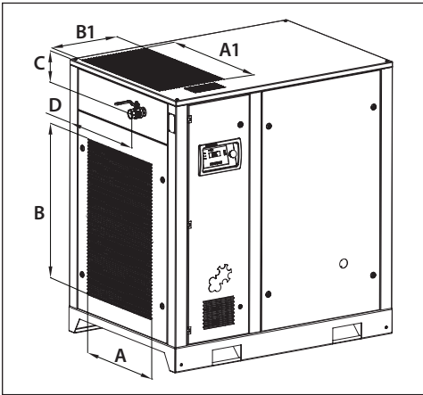
Fig. 3.3 Installation dimensions DV30-55
