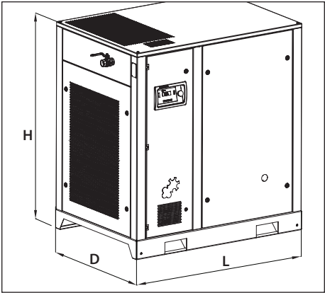
Fig. 3.2 Dimension drawing DV30-55
