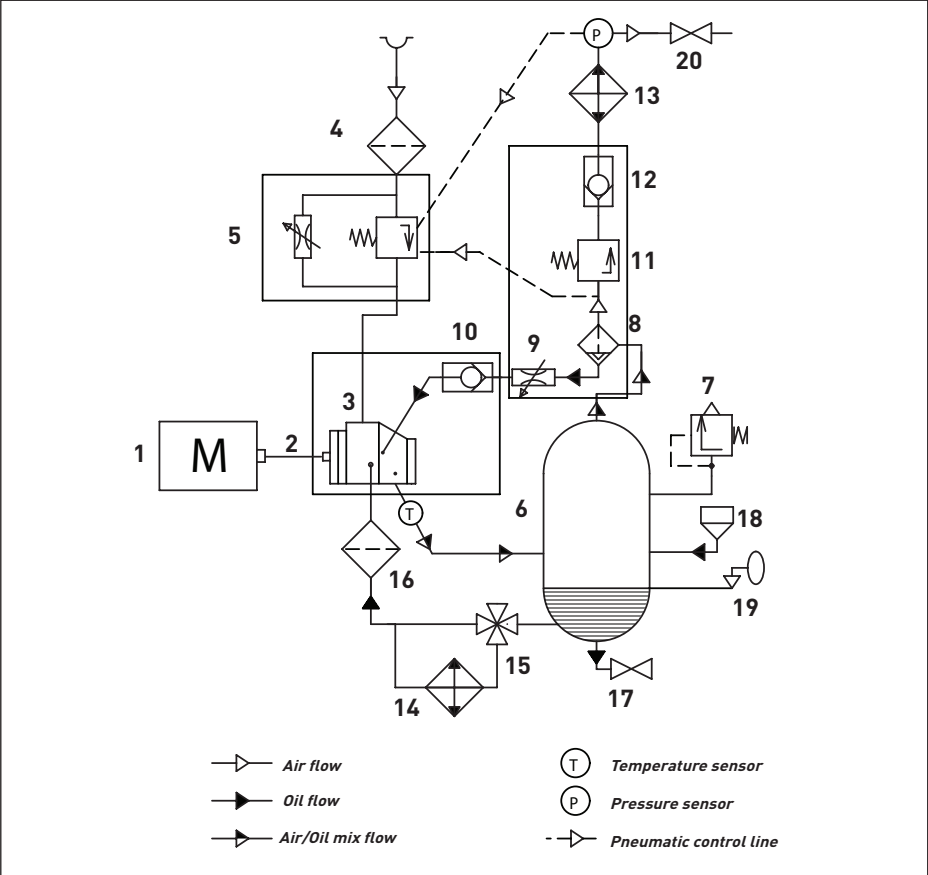
Fig. 2.3 Function diagram DV30-55
