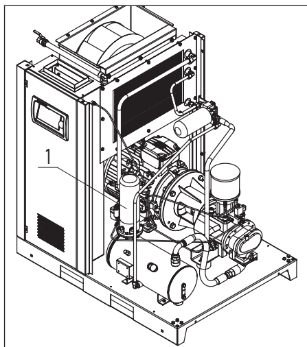
Fig. 5.5.2 Changing air-oil separator DV18 – DV22
