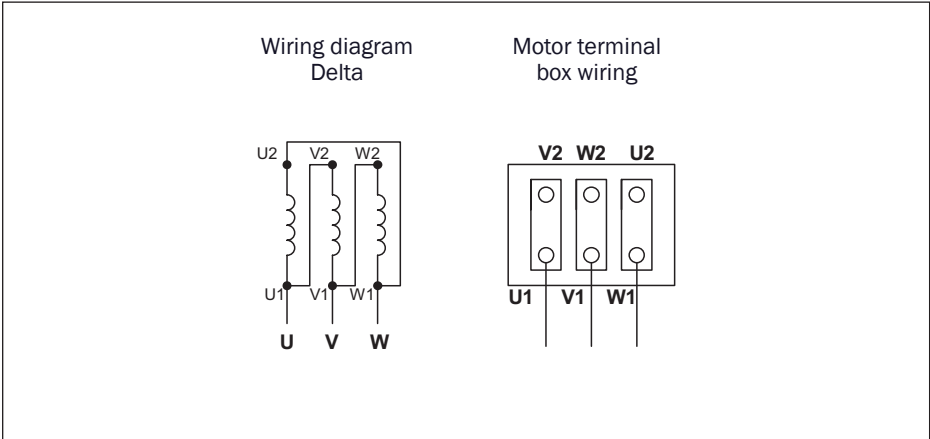
Fig. 2.6.2 Electric motor wiring diagram for DV11 – DV22
