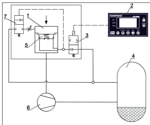
Fig. 2.5 Regulating system
