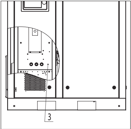
Fig. 3.6.2 Power cable terminal connection
