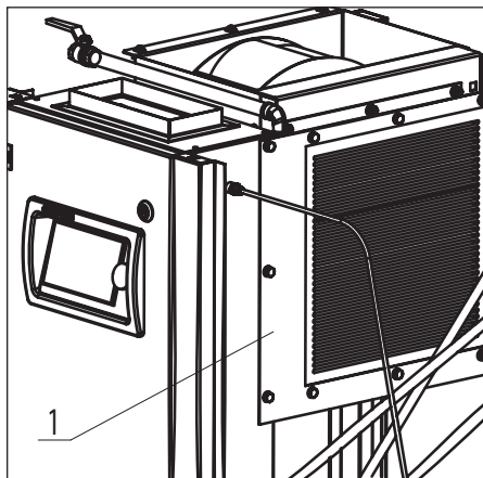
Fig. 5.6 Cleaning radiator
