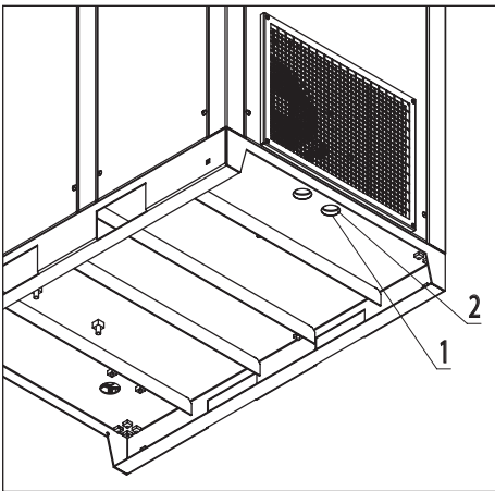
Fig. 3.6.1 Power cable connection
