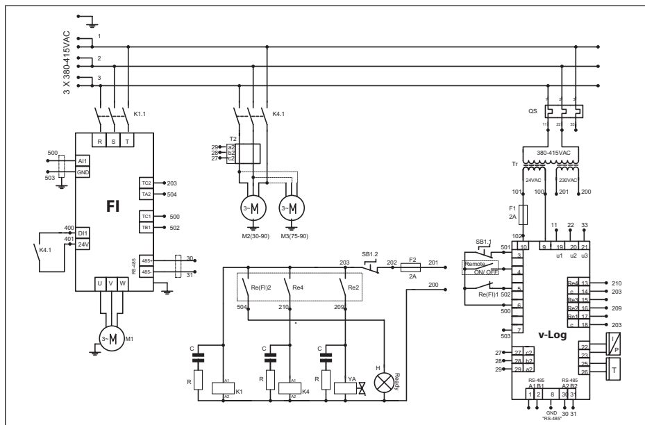
Fig. 2.6.1 Electrical diagram DV11 – DV22
