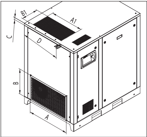
Fig. 3.3 Installation dimensions DV11 – DV22
