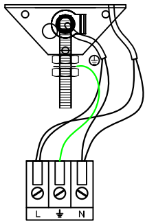
Figure:(The internal connection wire)
