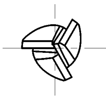
3 Flutes
