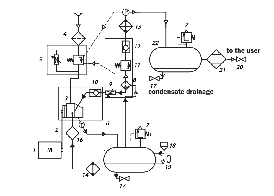
Fig. 2.3.2 Function diagram FR07...FRD22..., FRD07...FRD22..
