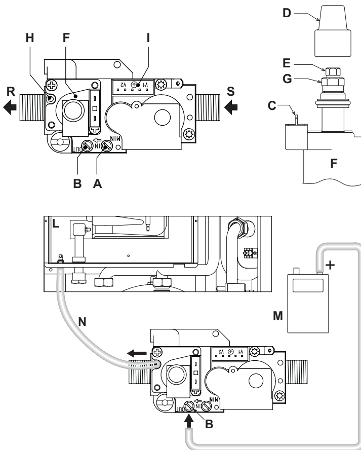
fig. 27 - Gas valve
