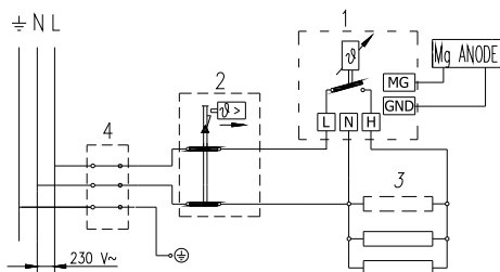
Electric installation
