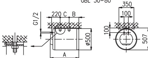
GBL 50-80
