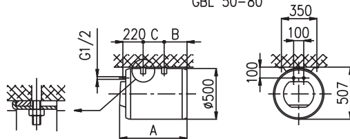
GBL 50–80
