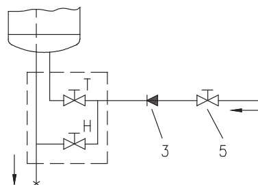
Open-circuit (gravity) system
