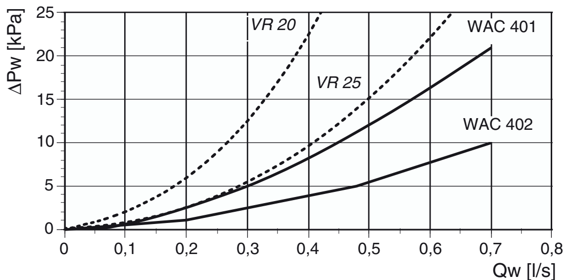
Pressure drop (water)
