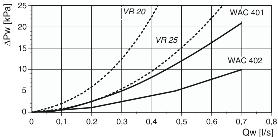
Pressure drop (water)
