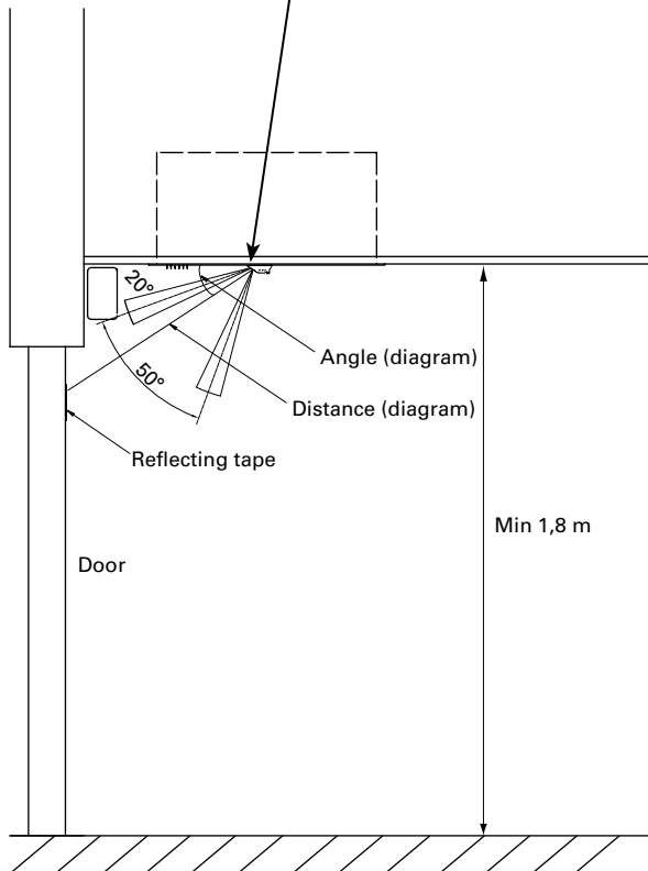
Fig. 6: Adjustment of the IR-eye downwards/upwards
