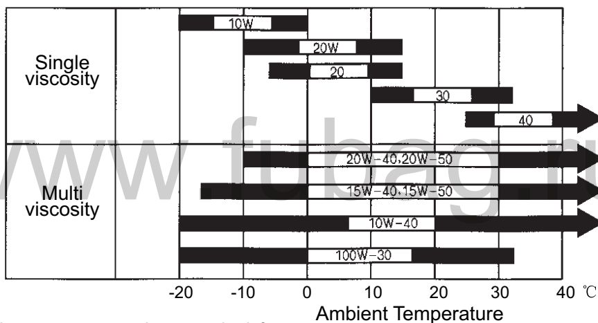
SAE Viscosity Grades
