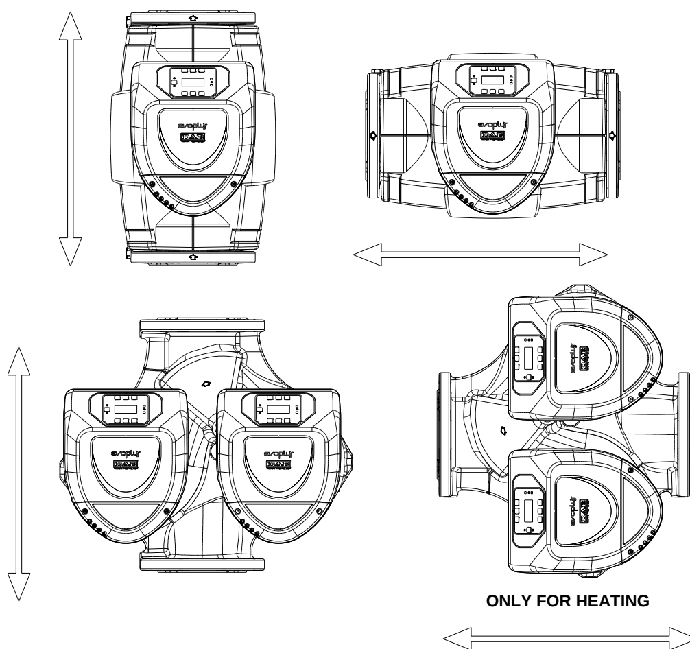
Figure 1: Assembly position
