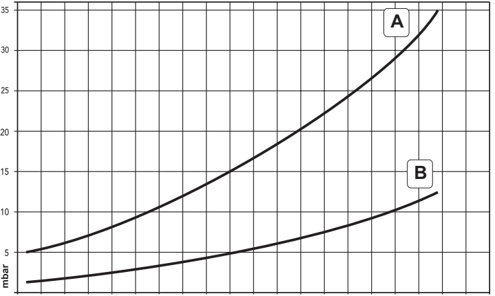
fig. 33 - Pressure/power diagram DIVAtop MICRO F 24
