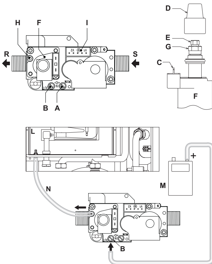
fig. 27 - Gas valve
