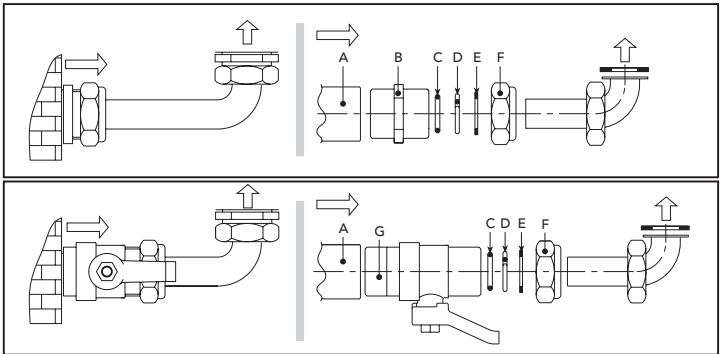
fig. 18 - Connection kit
