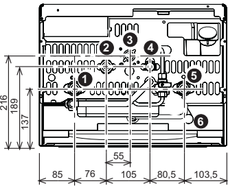
fig. 17 - Plumbing connections
