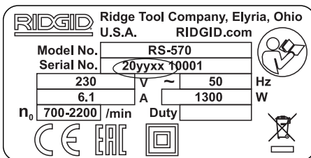
Figure 3 – Serial Plate ("20yy" = Year of Manufacture. "xx" = Week of Manufacture)
