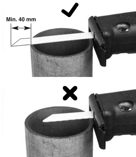
Figure 6 – Proper Blade Length
