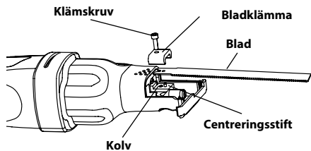
Figur 7 – Installera blad
