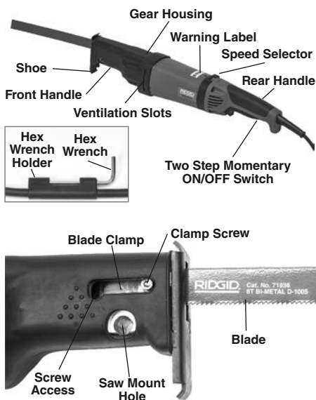
Figure 1 – RIDGID® RS-570 Reciprocating Saw
