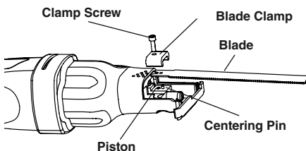
Figure 7 – Installing Blades
