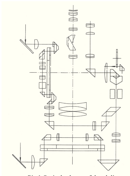
Pic.1 Optical scheme of theodolite
